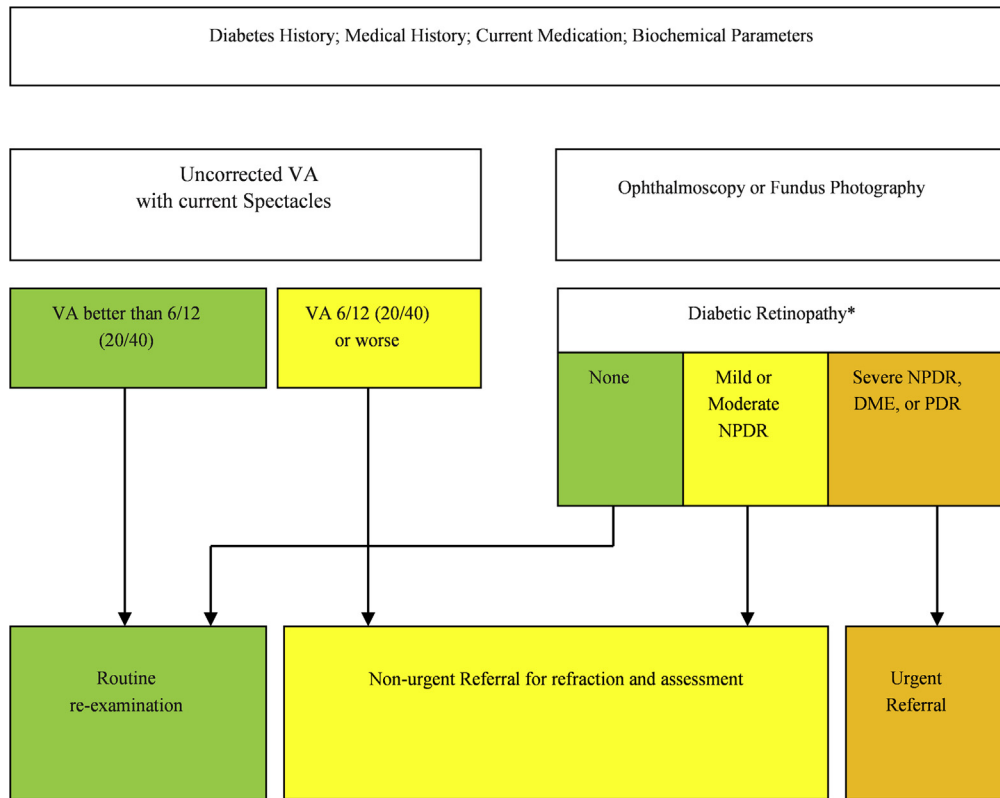
Figure 3. Flowchart showing screening for diabetic retinopathy. DME = diabetic macular edema; NPDR = nonproliferative diabetic retinopathy; PDR = proliferative diabetic retinopathy; VA = visual acuity. *Need to optimize medical treatment; glycemic control, hypertension, and lipids.
